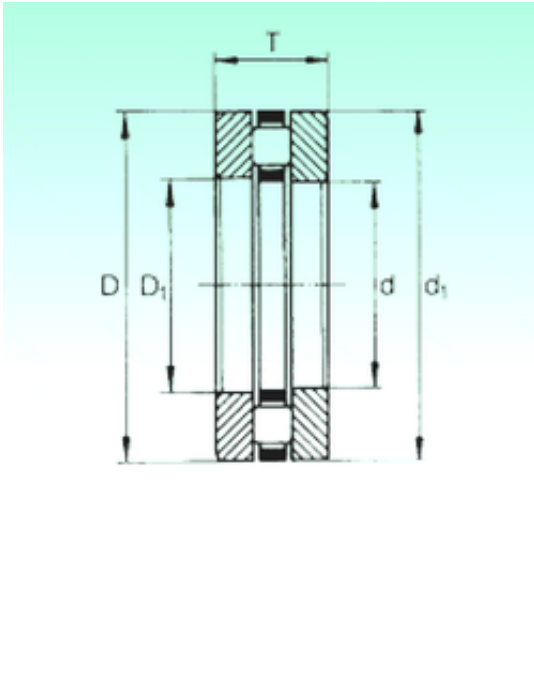
81222TN Bearing 2D drawings and 3D CAD models
