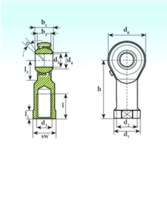
TSF 14 BB-O Bearing 2D drawings and 3D CAD models
